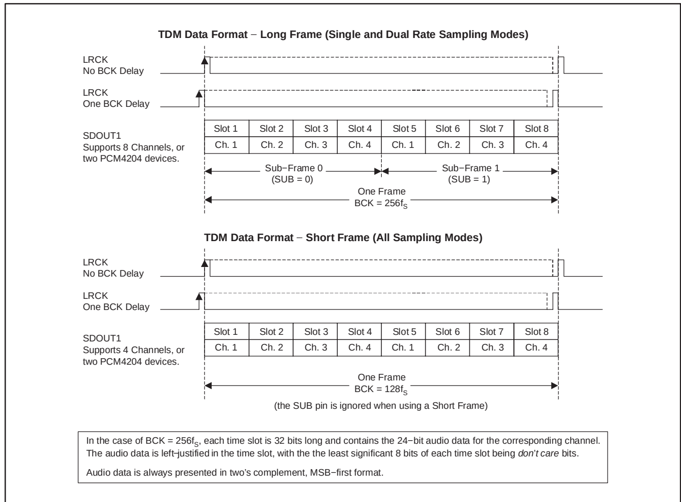
Figure 4. PCM Data Formats: Time Division Multiplexed (TDM)
